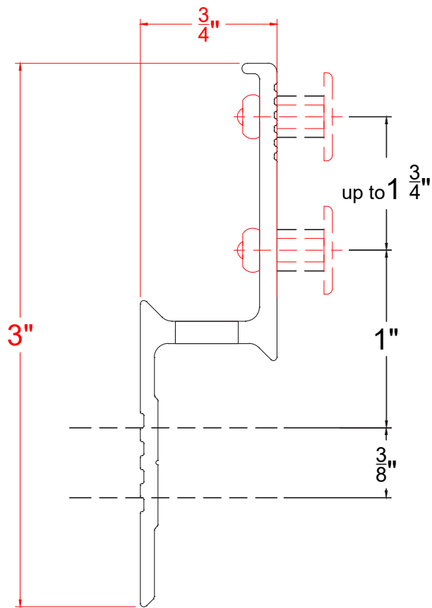
X-Z19PF PROFILE
